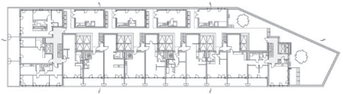
Fourth floor
