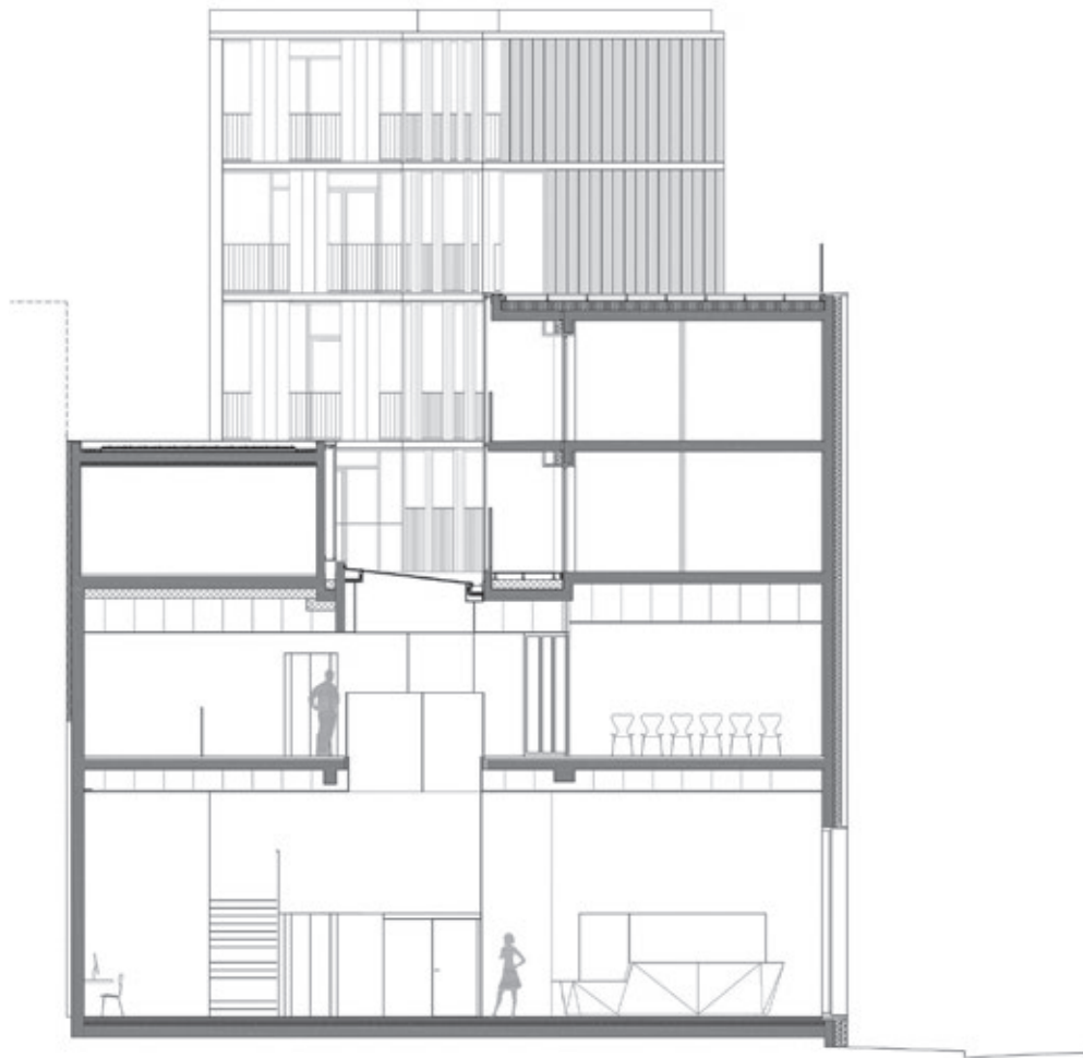
Section 0 1 5 10
